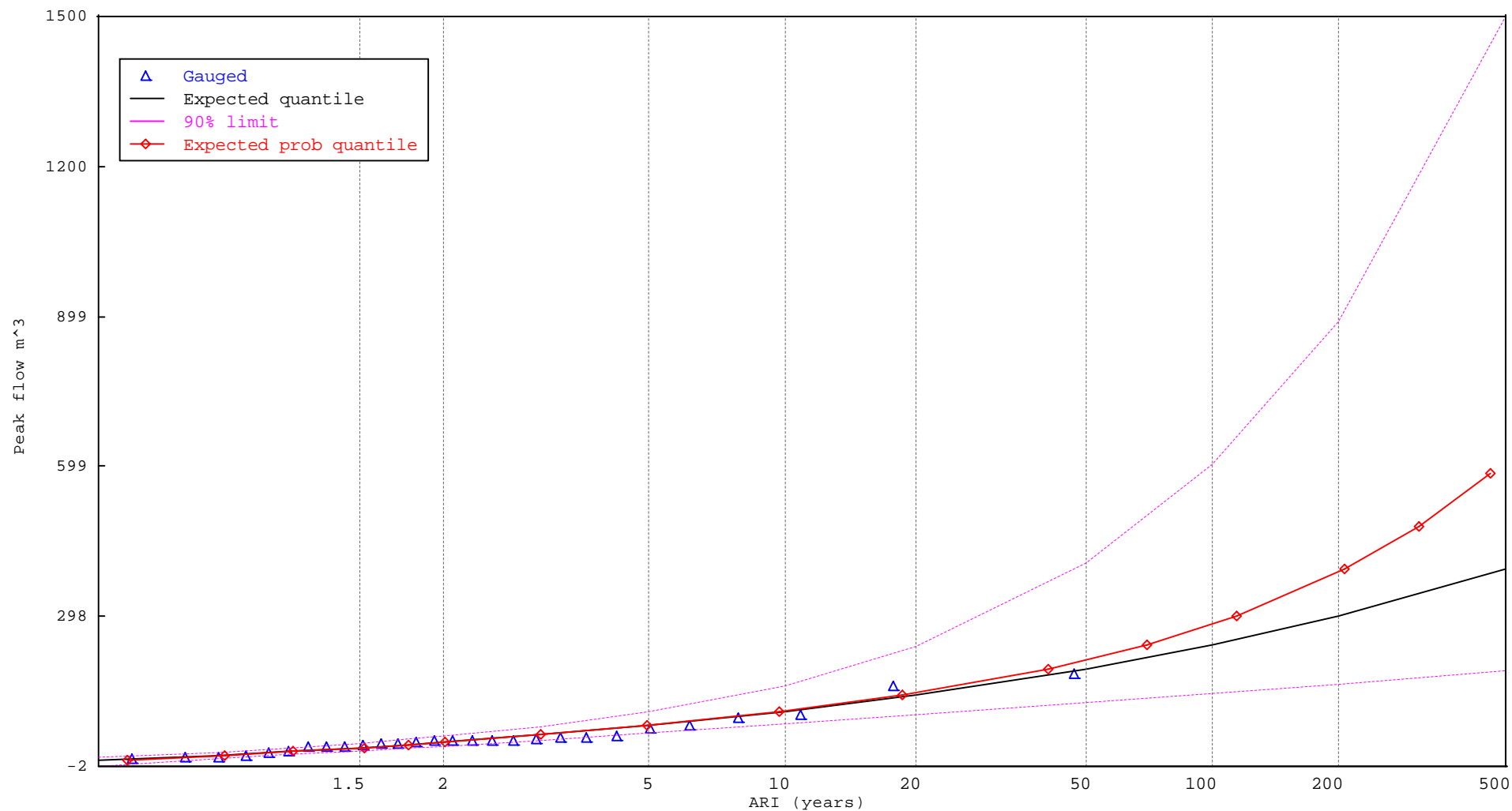
Figure C.3 Generalised Extreme Value flood frequency assessment (10 lowest annual flows removed)
