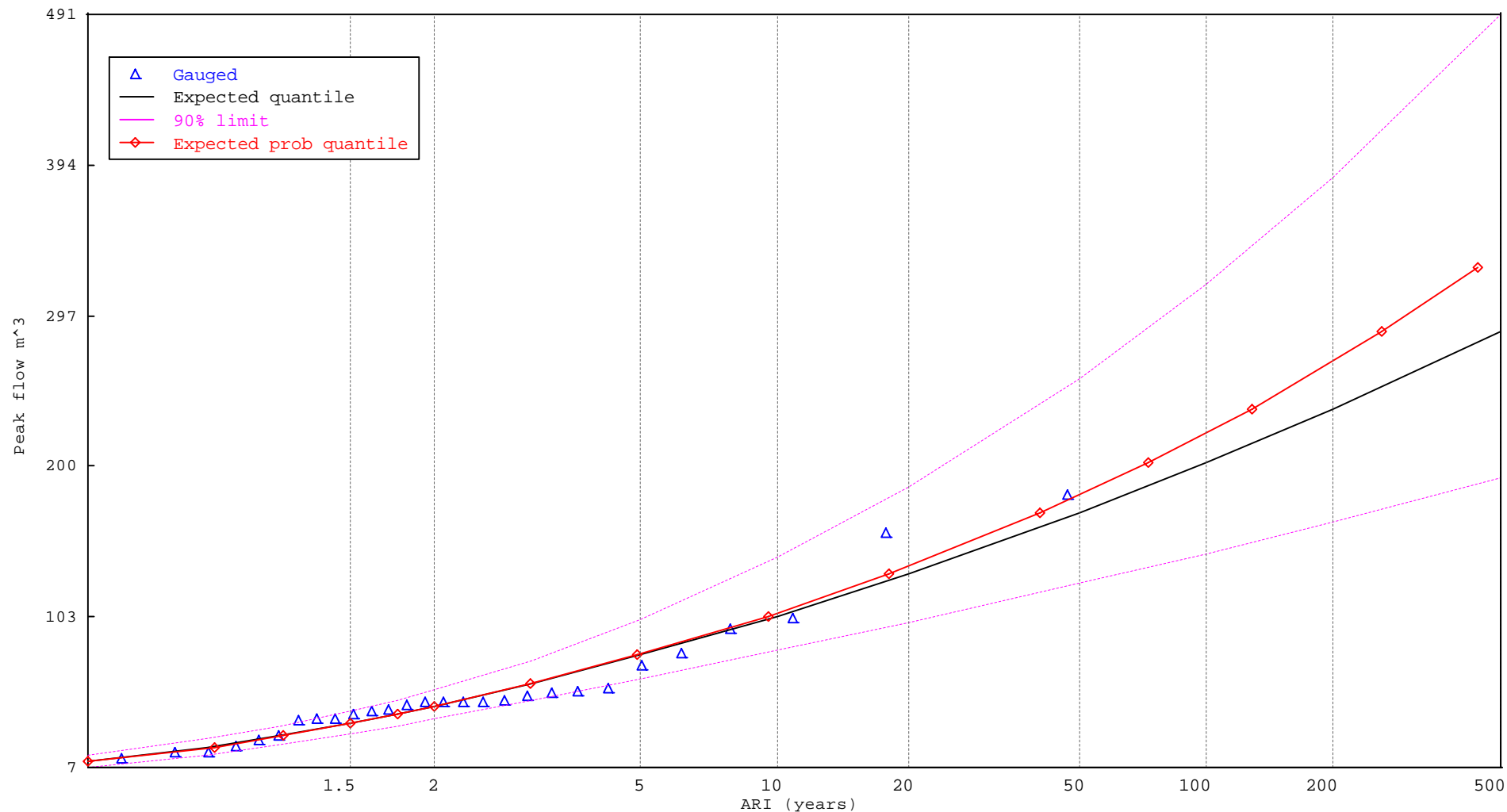
Figure C.1 Log-Normal flood frequency assessment (10 lowest annual flows removed)
