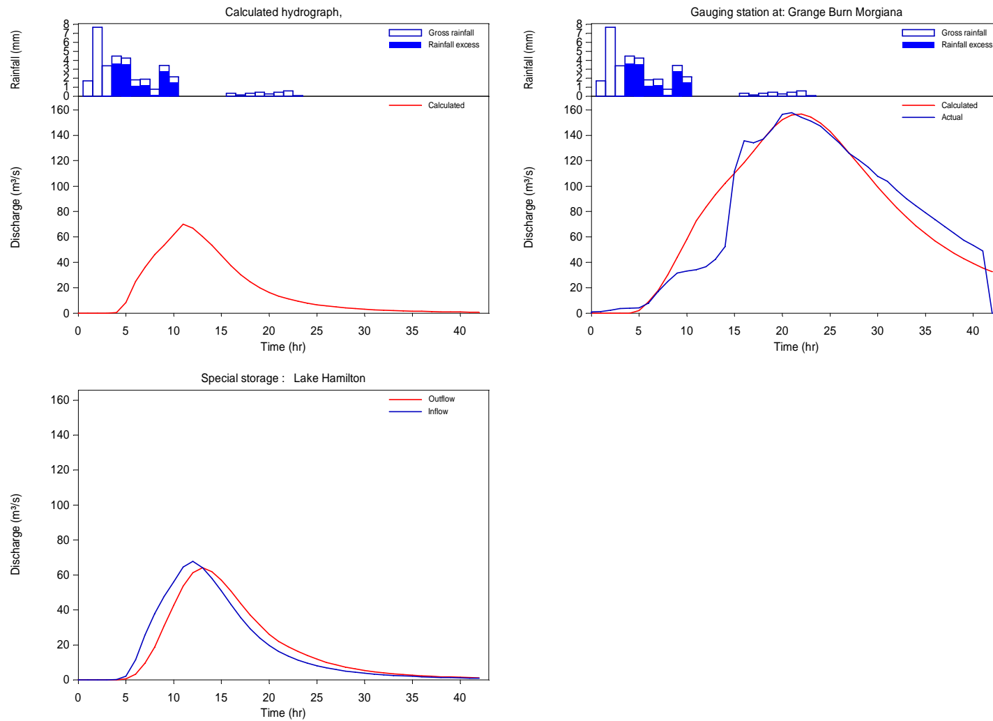
Figure B.3 Calibrated Grange Burn model for the August 2004 event (Cardno, 2010)
