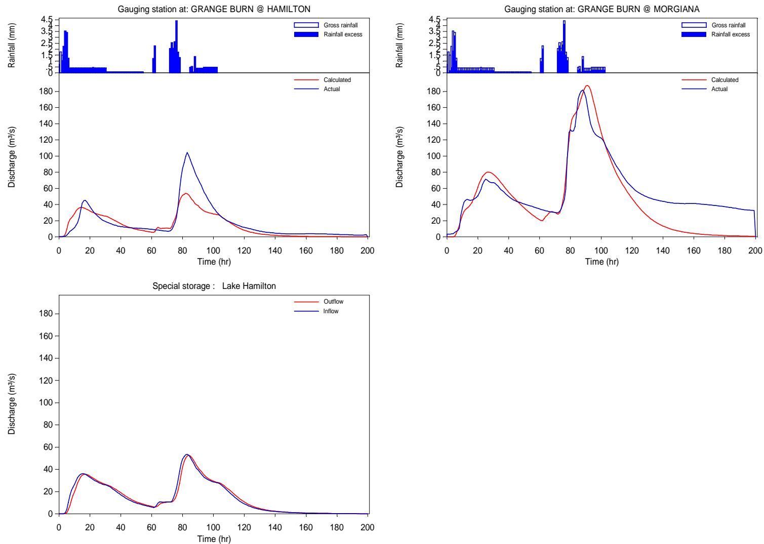
Figure B.1 Calibrated Grange Burn model for the September 1983 event (Cardno, 2010)
