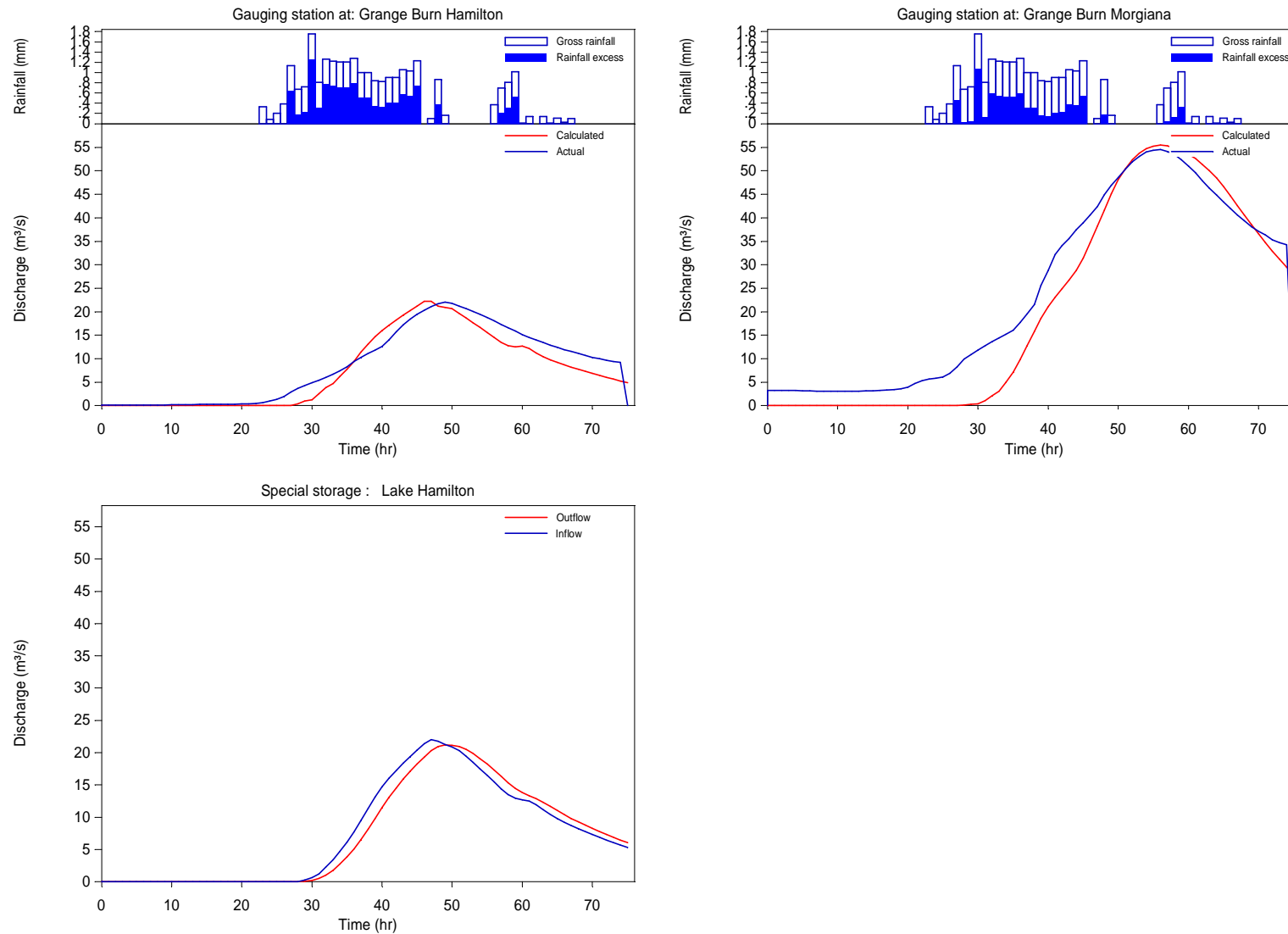
Figure B.2 Calibrated Grange Burn model for the September 1984 event (Cardno, 2010)
