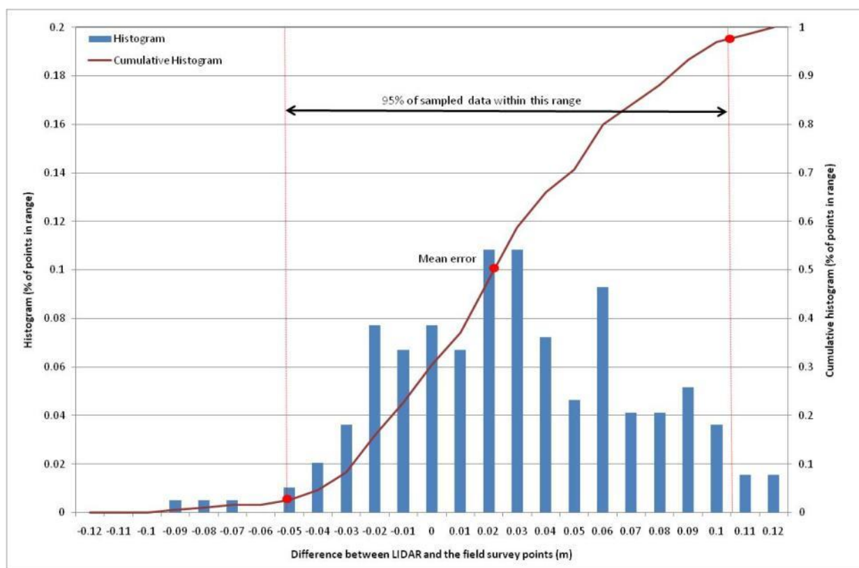
Figure 3.3 Analysis of the difference between the 2011 LiDAR data and field survey
