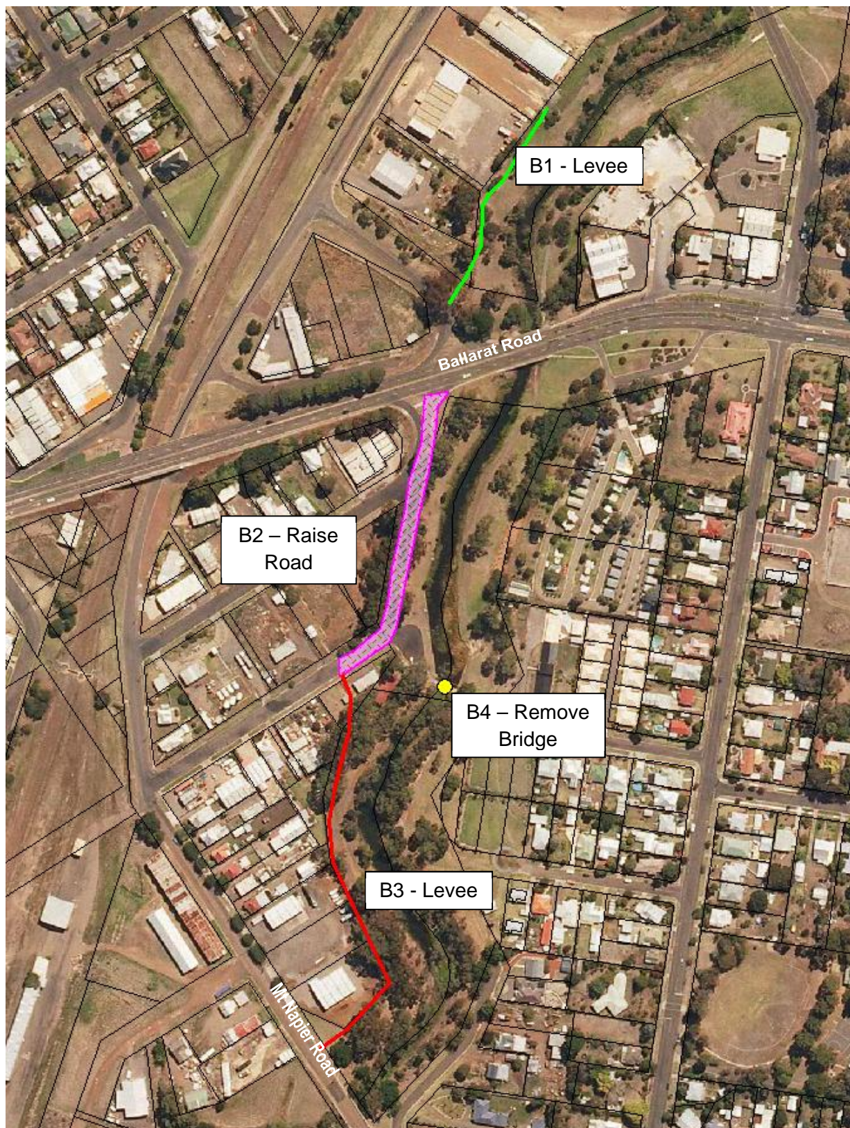
Figure 8.4 Model B – Grange Burn mitigation options
