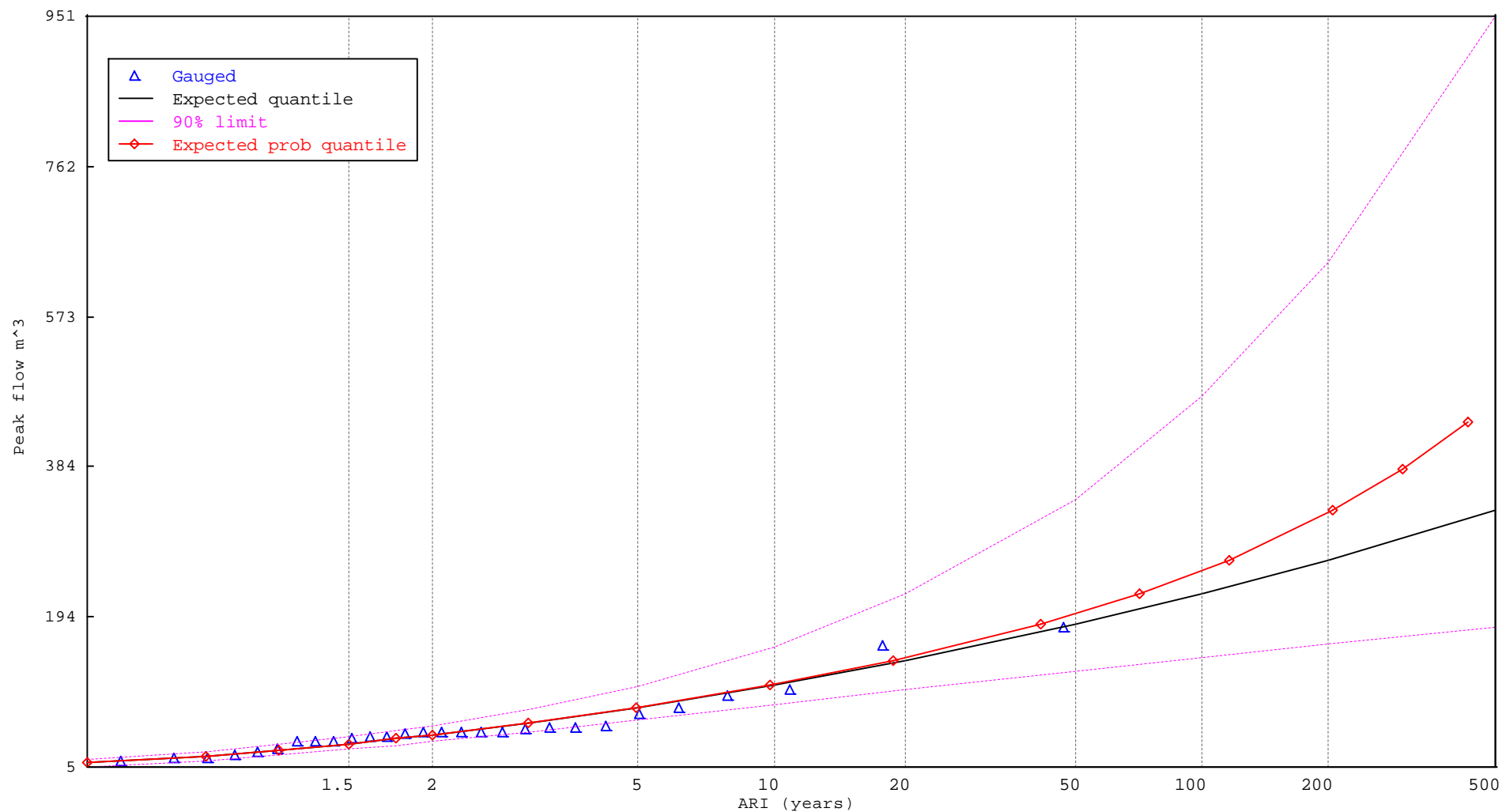
Figure C.2 Log Pearson Type III flood frequency assessment (10 lowest annual flows removed)
