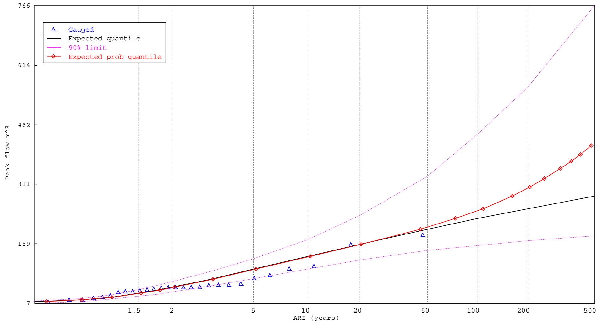
Figure C.4 Generalised Pareto flood frequency assessment (10 lowest annual flows removed)
