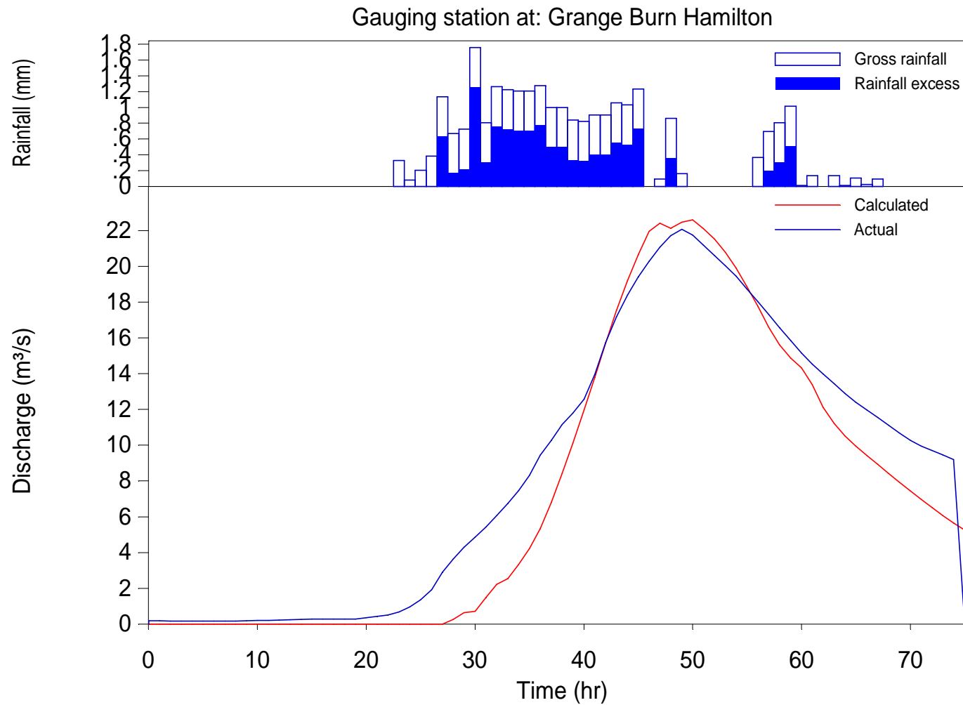
Figure B.6 Calibrated Grange Burn model for the September 1984 event
