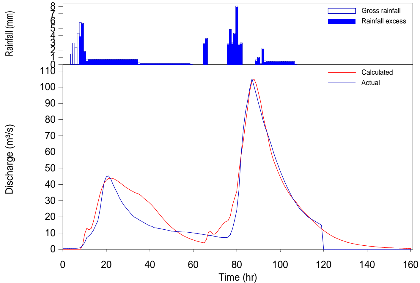
Figure B.4 Calibrated Grange Burn model for the September 1983 event (full event)
