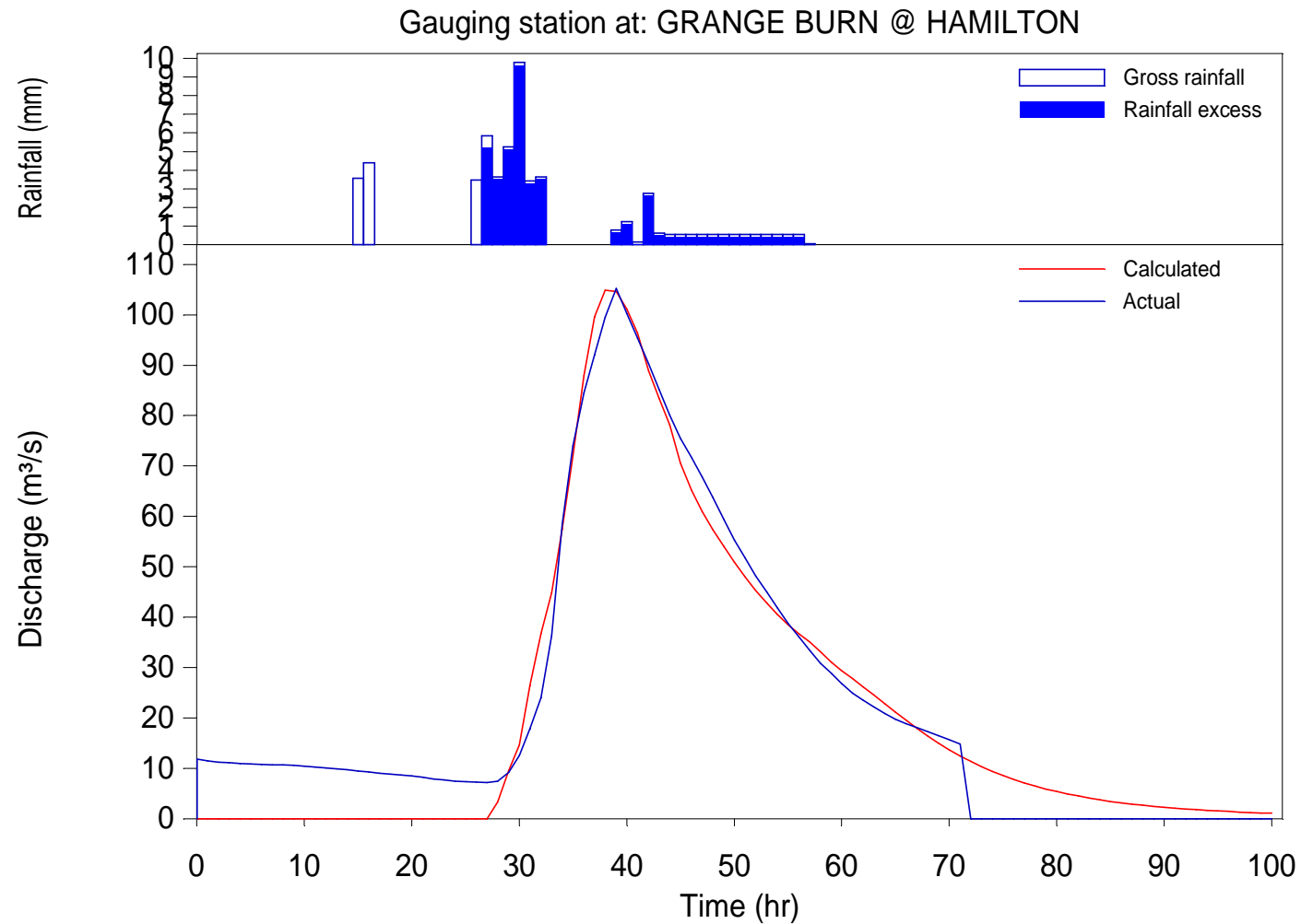
Figure B.5 Calibrated Grange Burn model for the September 1983 event (isolated peak)
